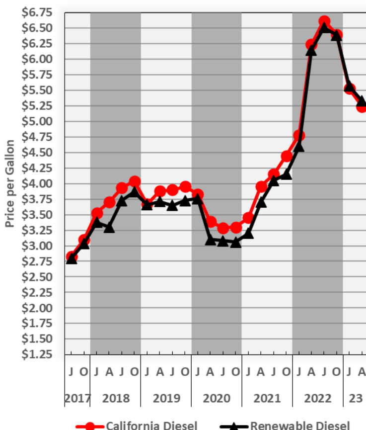
FIGURE 16 HISTORICAL RENEWABLE DIESEL PRICES VERSUS DIESEL (CALIFORNIA DATA ONLY)
